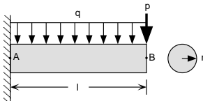
Figure: Cantilever Beam
